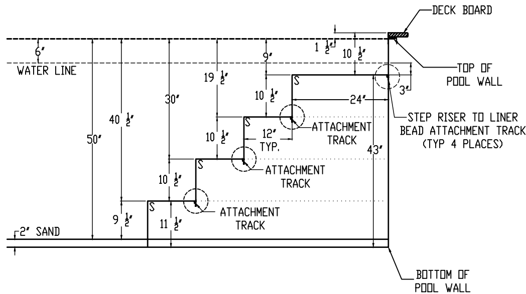
STEP RISER TO LINER BEAD ATTACHMENT TRACK DETAIL
