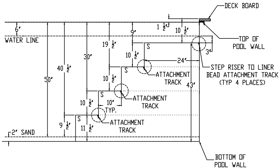
STEP RISER TO LINER BEAD ATTACHMENT TRACK DETAIL
