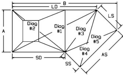
Figure 1 Angled Transition
