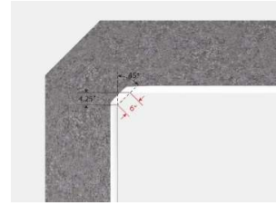
Cut-Off (Diagonal)
